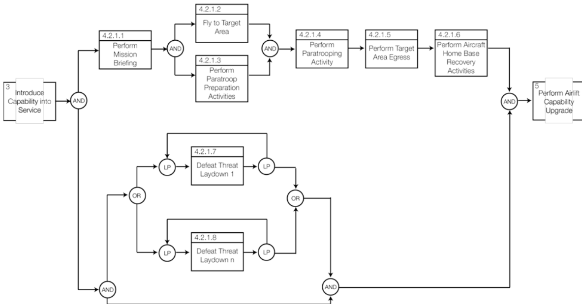
Figure 5: Functional Flow Block Diagram
