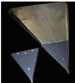
G-16 Former Nose and Board
