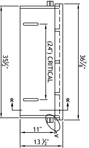
HOOD ELEVATION
