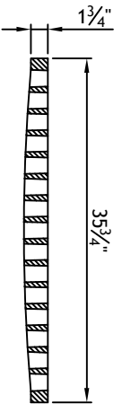
SECTION A-A (GRATE)
