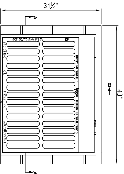
PLAN (FRAME & GRATE)
