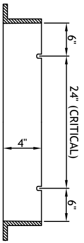
SECTION K-K
