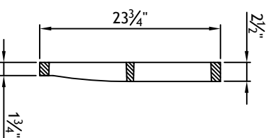
SECTION B-B (GRATE)
