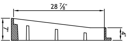
SECTION J-J
