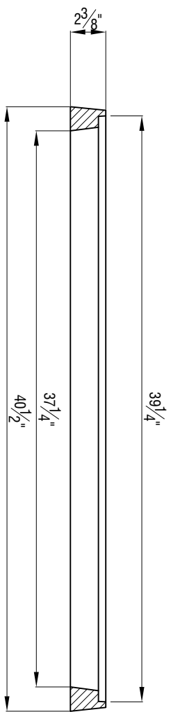
SECTION " A - A "
