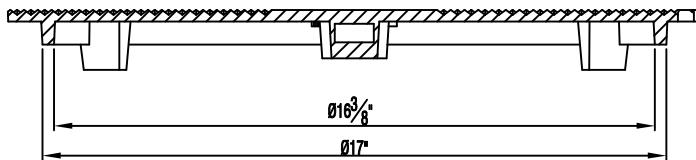
SECTION " A - A "
