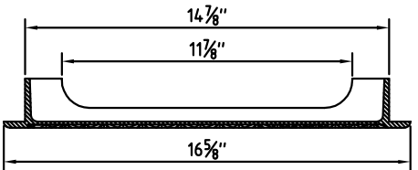
ELEVATION SECTION - BB
