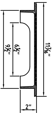
SIDE VIEW SECTION - AA
