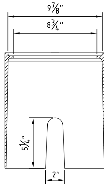
SECTION BB
