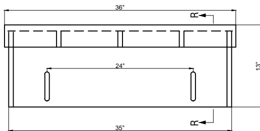
HOOD ELEVATION
