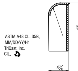
SECTION R-R
