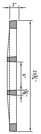
GRATE SECTION A-A
