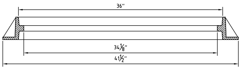
FRAME SECTION B-B
