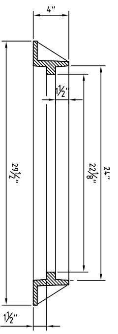
FRAME SECTION A-A
