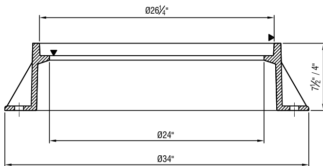
FRAME SECTION - XX
